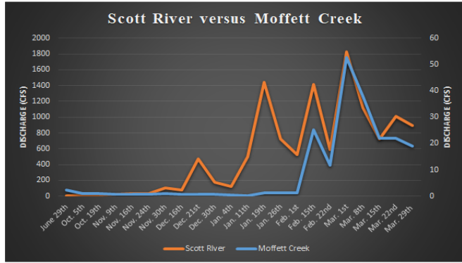
Figure 11: Moffett Creek and Scott River flow data from 2018-2019.
