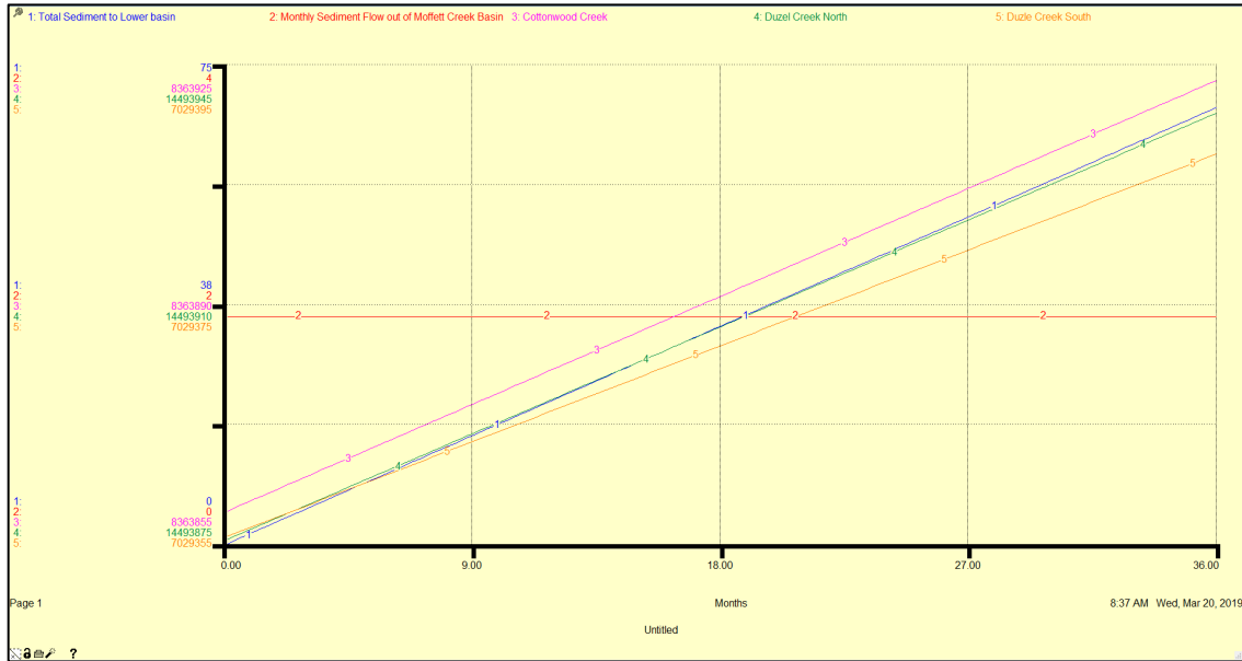
Figure 8: Stella model results. Line 2 is sediment delivered out of watershed. Lines 1, 3, 4, 5 are sediment amounts for each modelled sub-basin.
